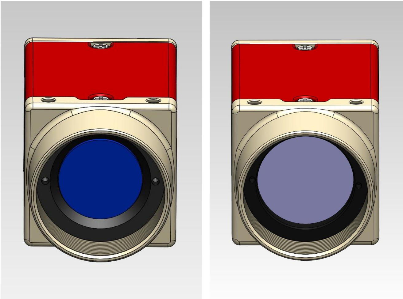
Figure1: Mako-G camera with 16mm metal (left image) and 22mm plastic (right image) filter mount
