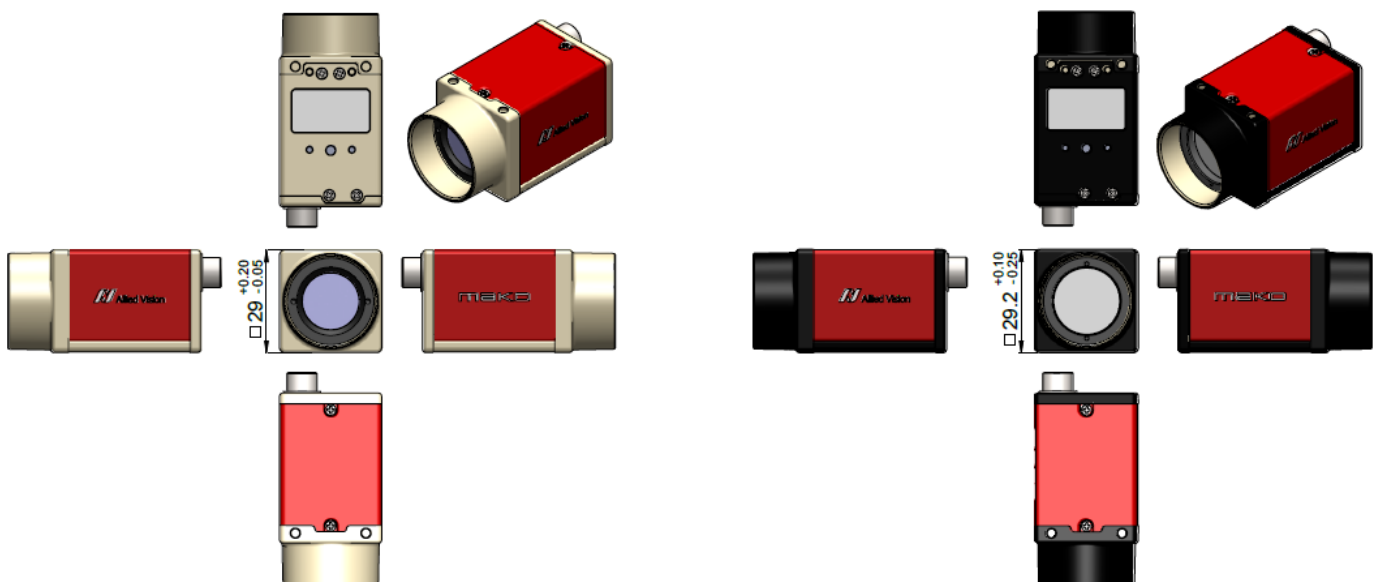
Figure 1 – Front flange dimension of old silver nickel plating vs. new black powder coating
