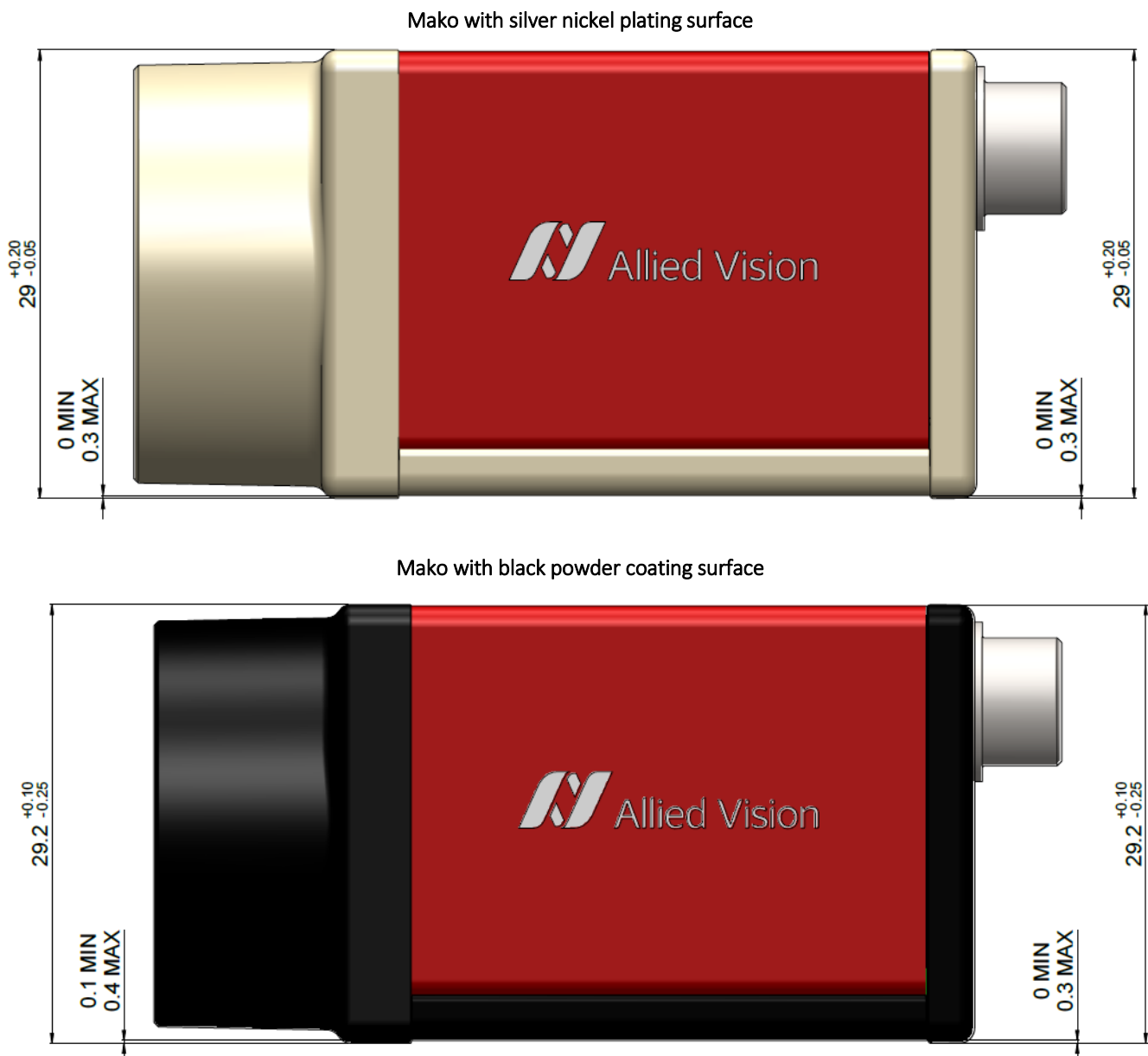
Figure 2 – Front flange and back plate vs. bottom plate: housings with legacy silver nickel plating vs. new black powder coating
