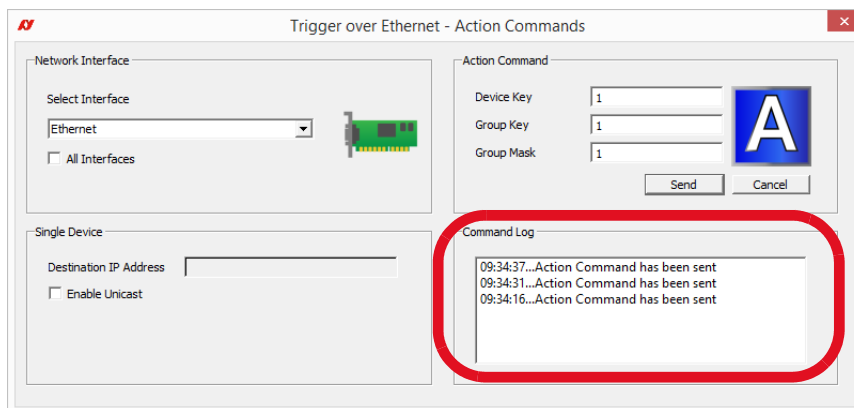
Figure 5: Command log
